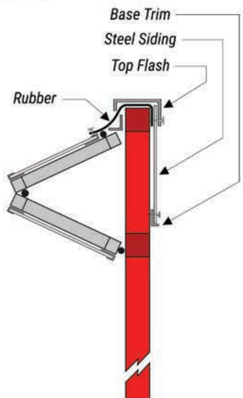
Side View of Flashing
